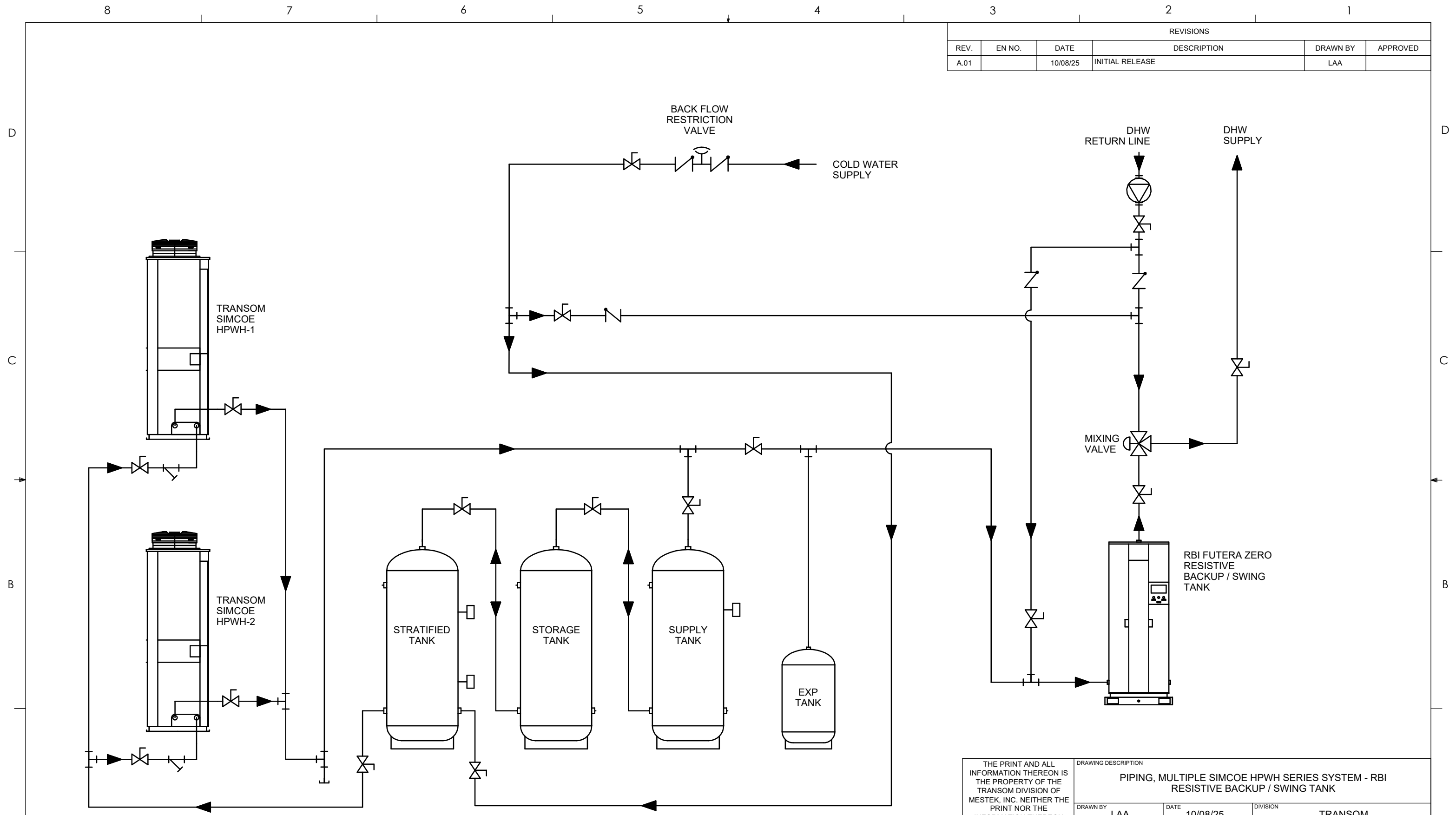
(PIPING, MULTIPLE SIMCOE HPWH SERIES SYSTEM - RBI RESISTIVE BACKUP / SWING TANK) SHOWN
